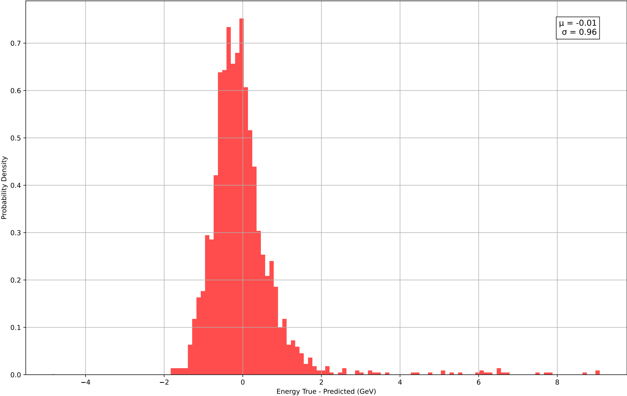
Energy Residuals (10.0-11.0 GeV)
