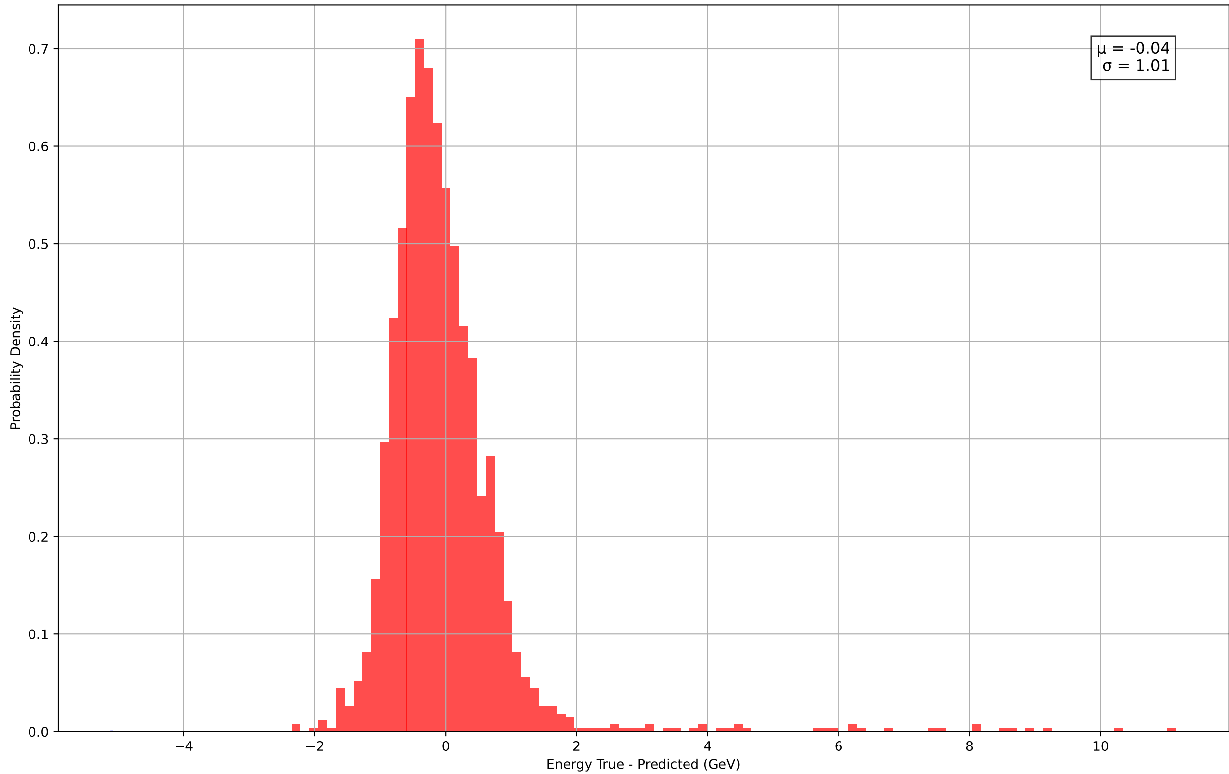
Energy Residuals (12.0-13.0 GeV)
