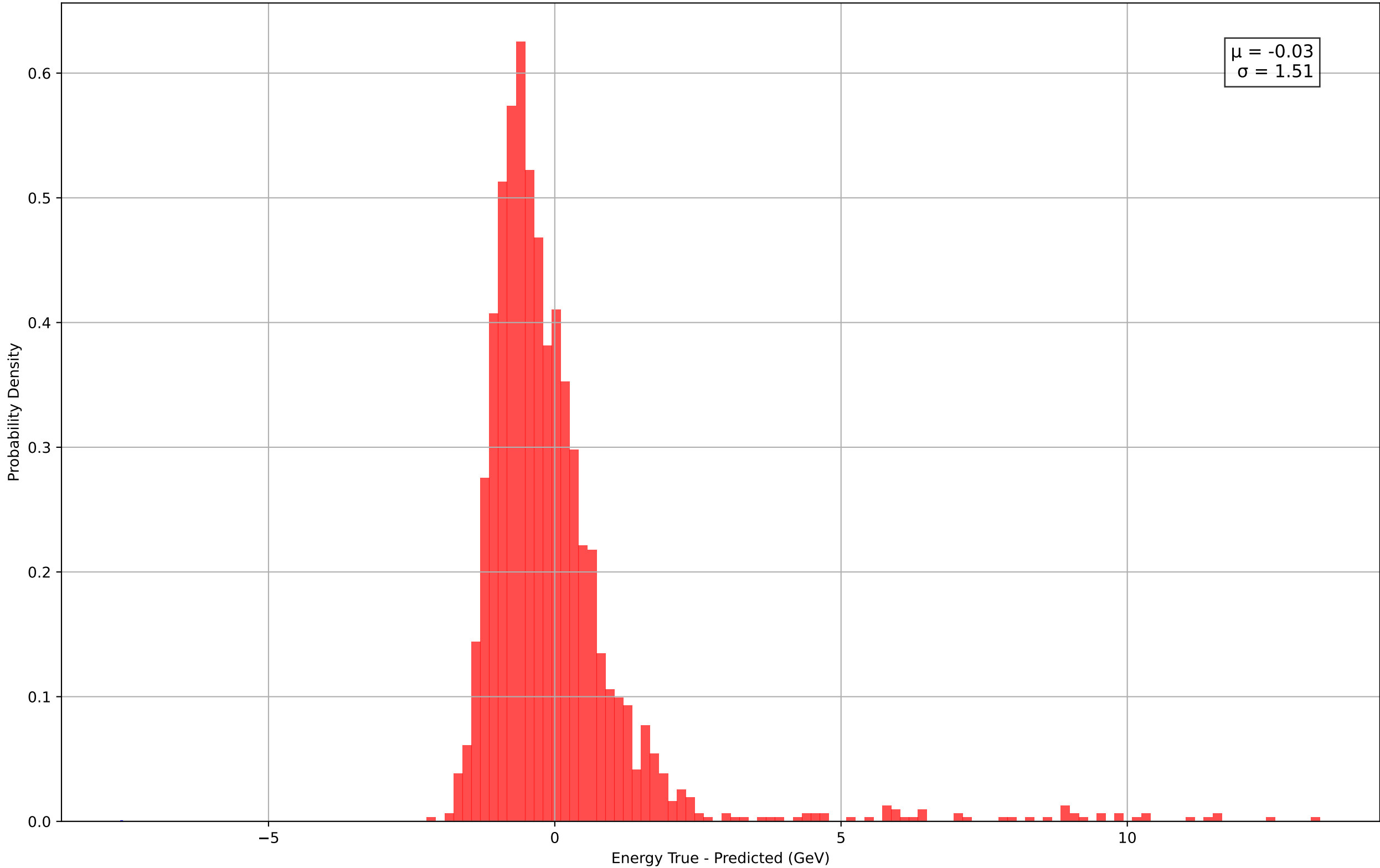
Energy Residuals (17.0-18.0 GeV)
