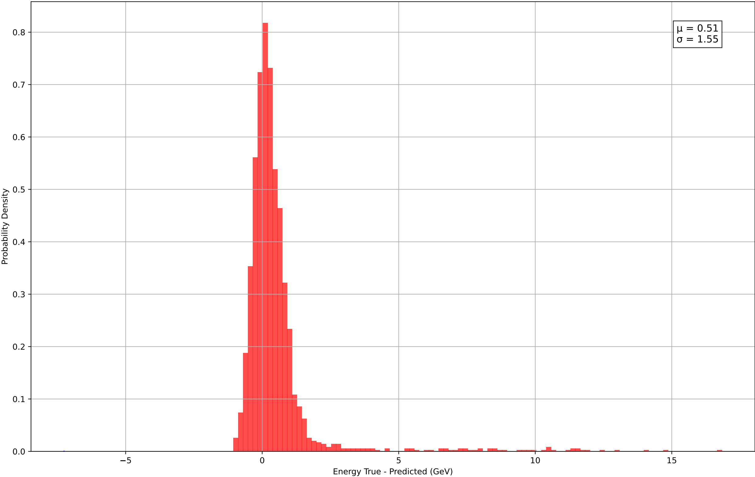
Energy Residuals (19.0-20.0 GeV)
