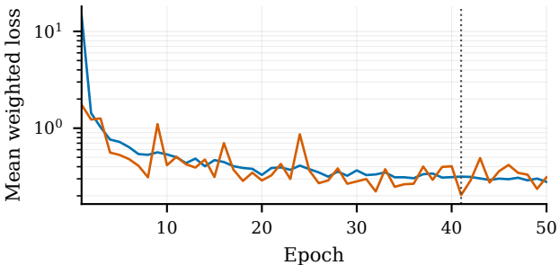
Learned decoder: k_1\mathcal{L}_1
