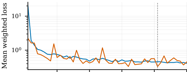
Combined objective
