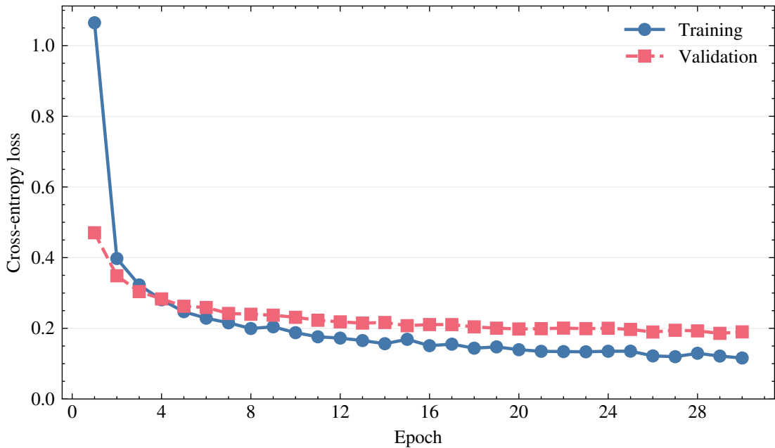
ResNet50 vehicle classification
