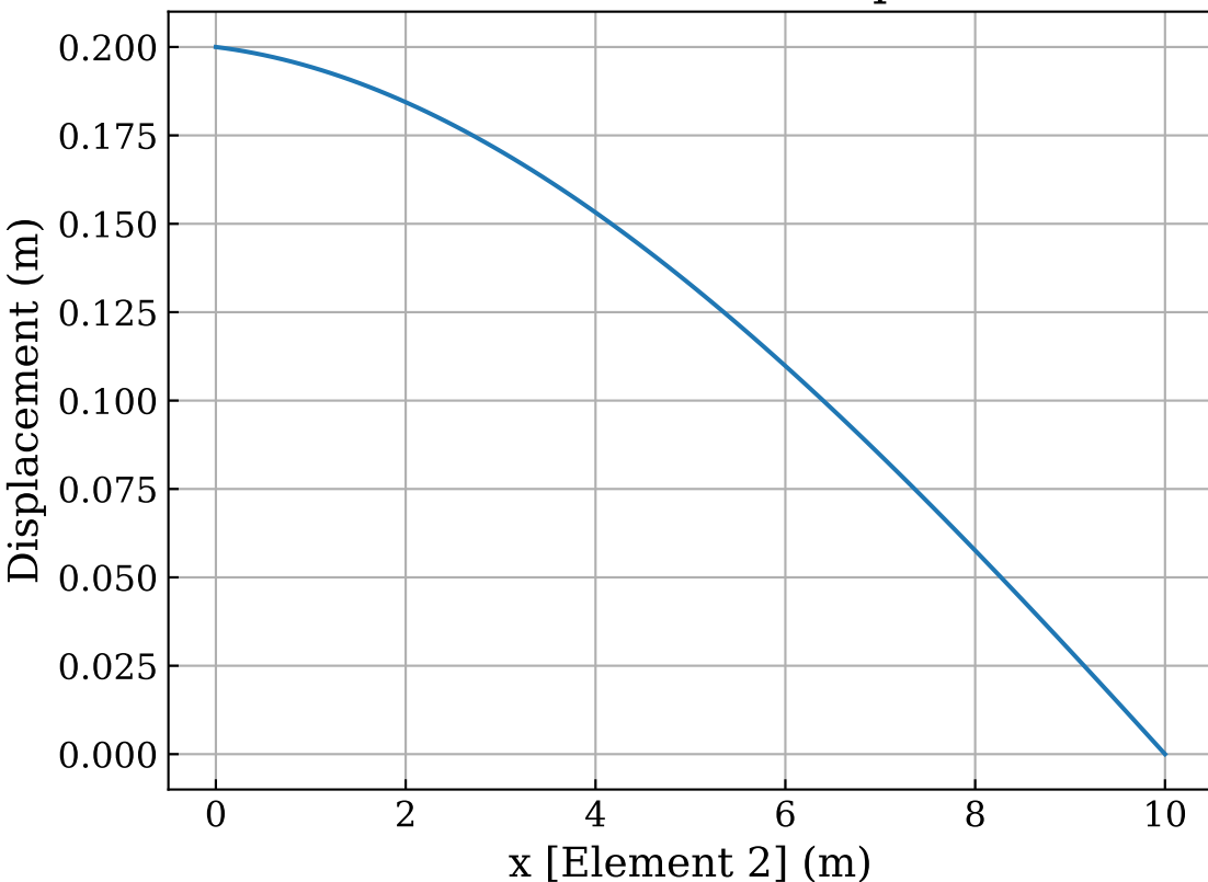
Element 2 Transverse Displacement
