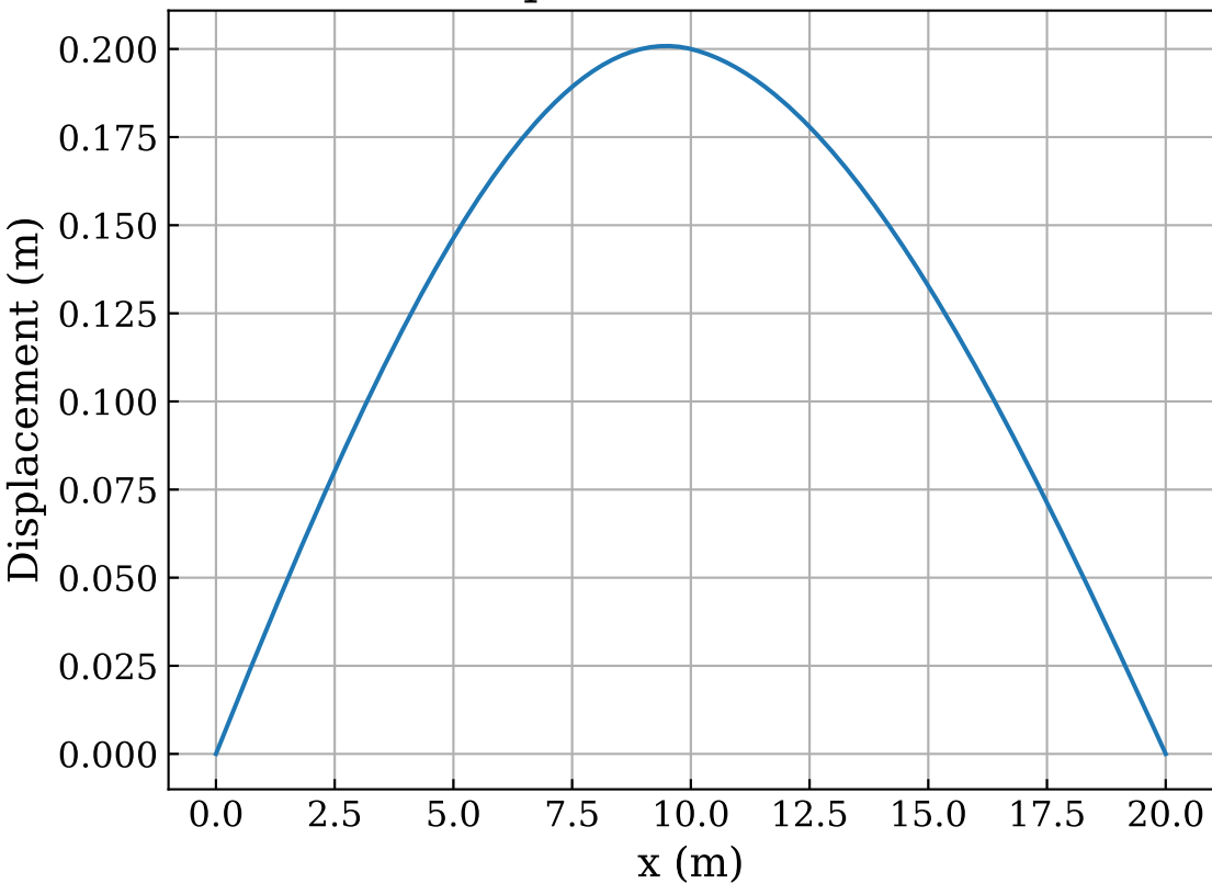
Transverse Displacement Over Entire Beam
