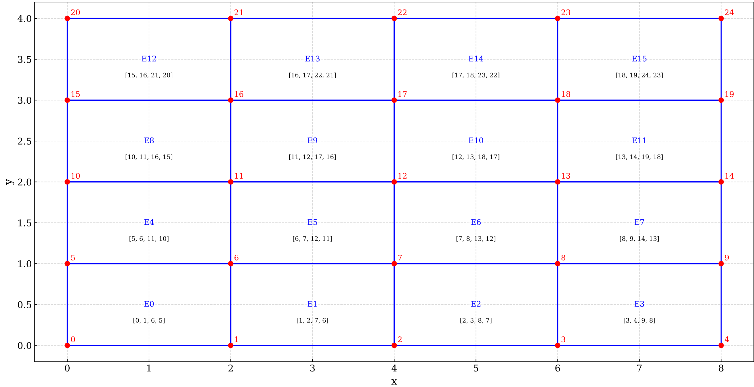
2D Quadrilateral Grid: Node and Element Labels
