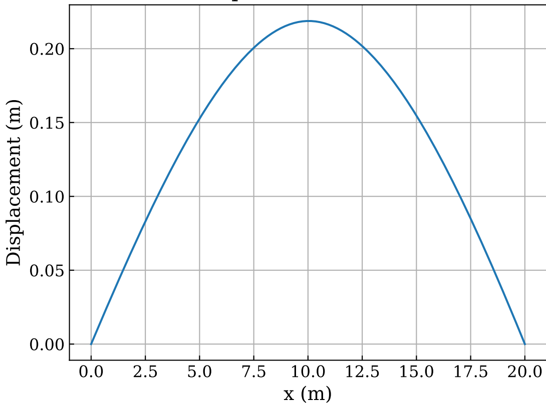
Transverse Displacement Over Entire Beam
