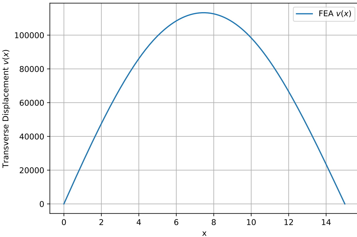
FEA Solution for v(x)
