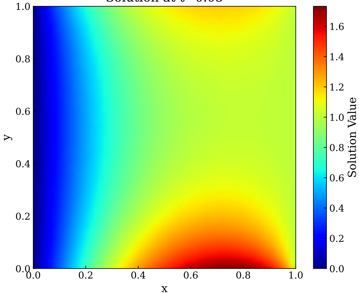
Solution at t=0.05
