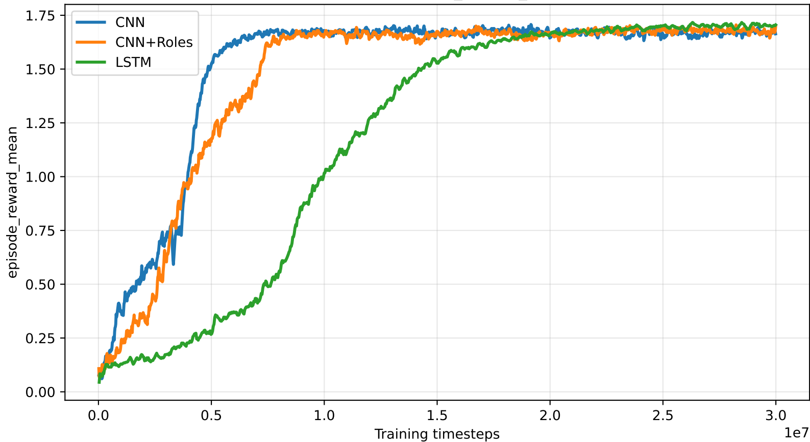
Training comparison:S1 episode_reward_mean rolling mean
