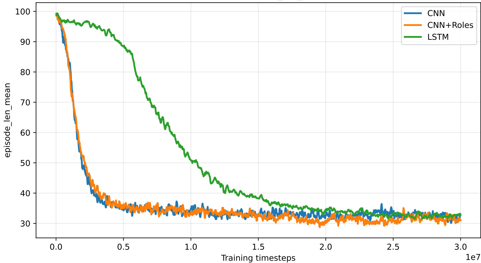
Training comparison:S2 episode_len_mean rolling mean
