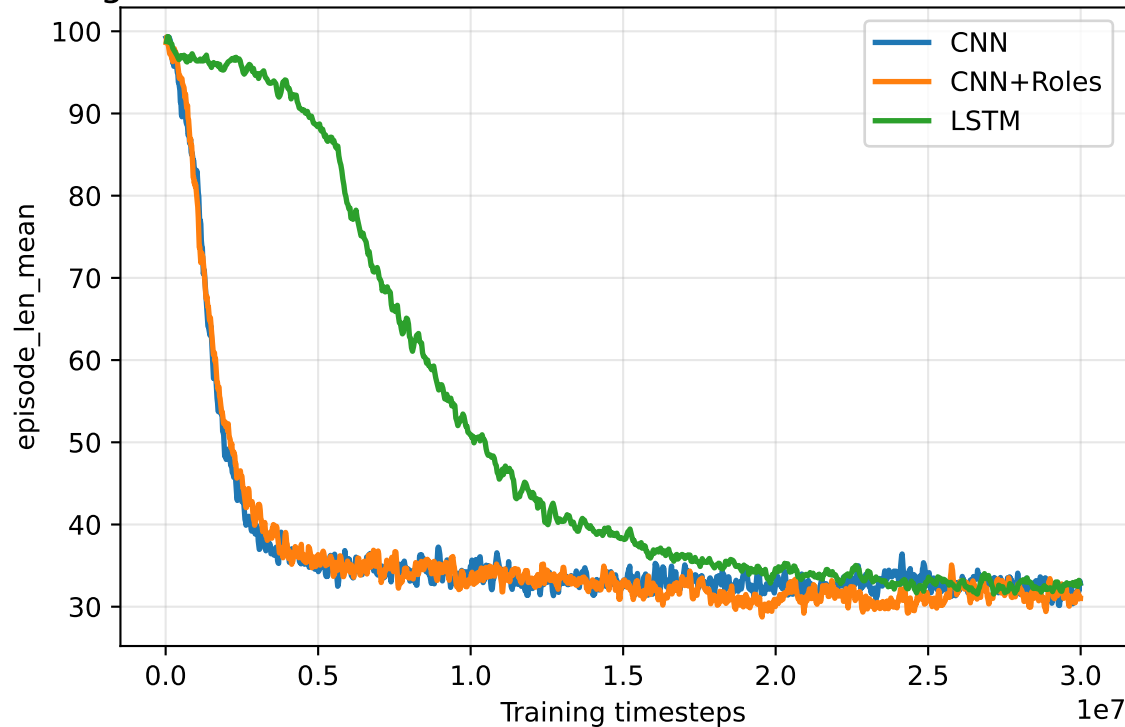
episode_reward_training run comparison, rolling mean window = 5episode_len_mean
