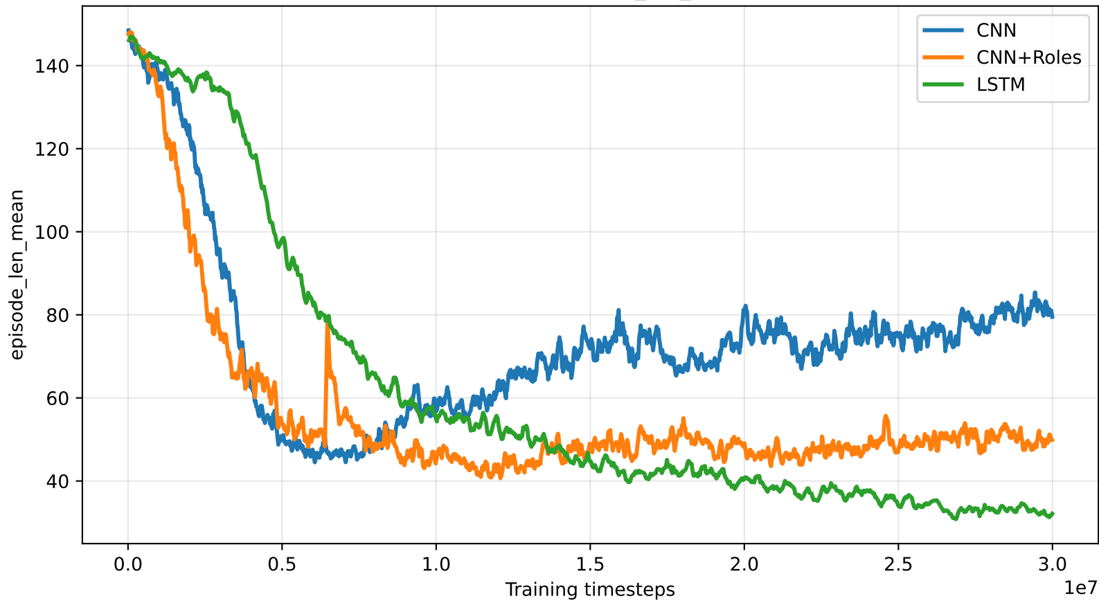
Training comparison:S3 episode_len_mean rolling mean
