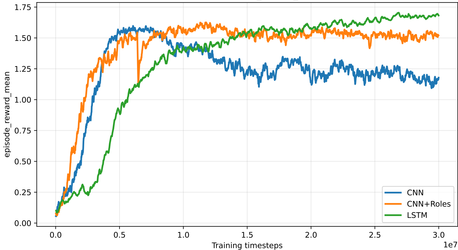
Training comparison:S3 episode_reward_mean rolling mean
