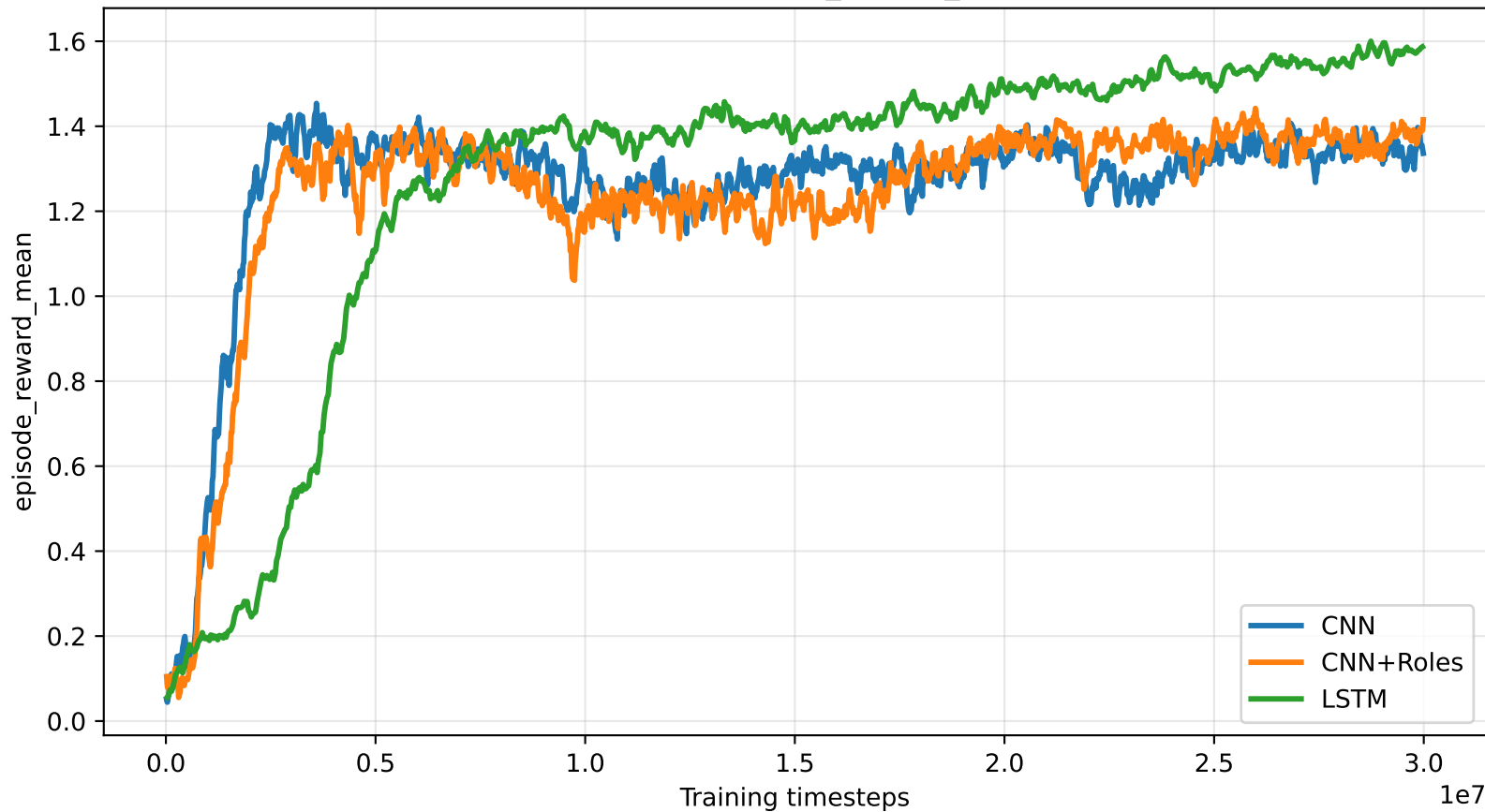
Training comparison:S4 episode_reward_mean rolling mean
