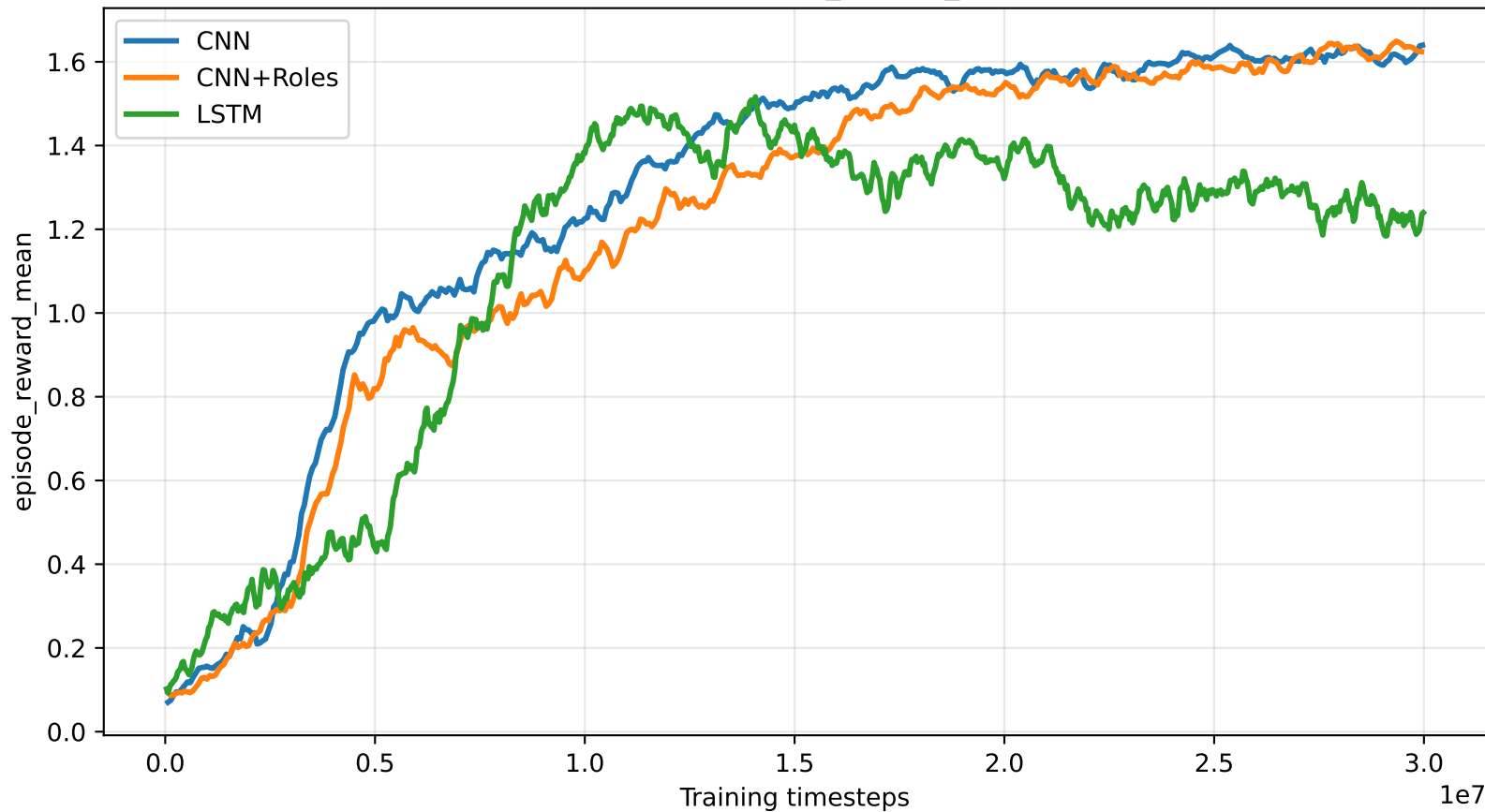
Training comparison:S5 episode_reward_mean rolling mean
