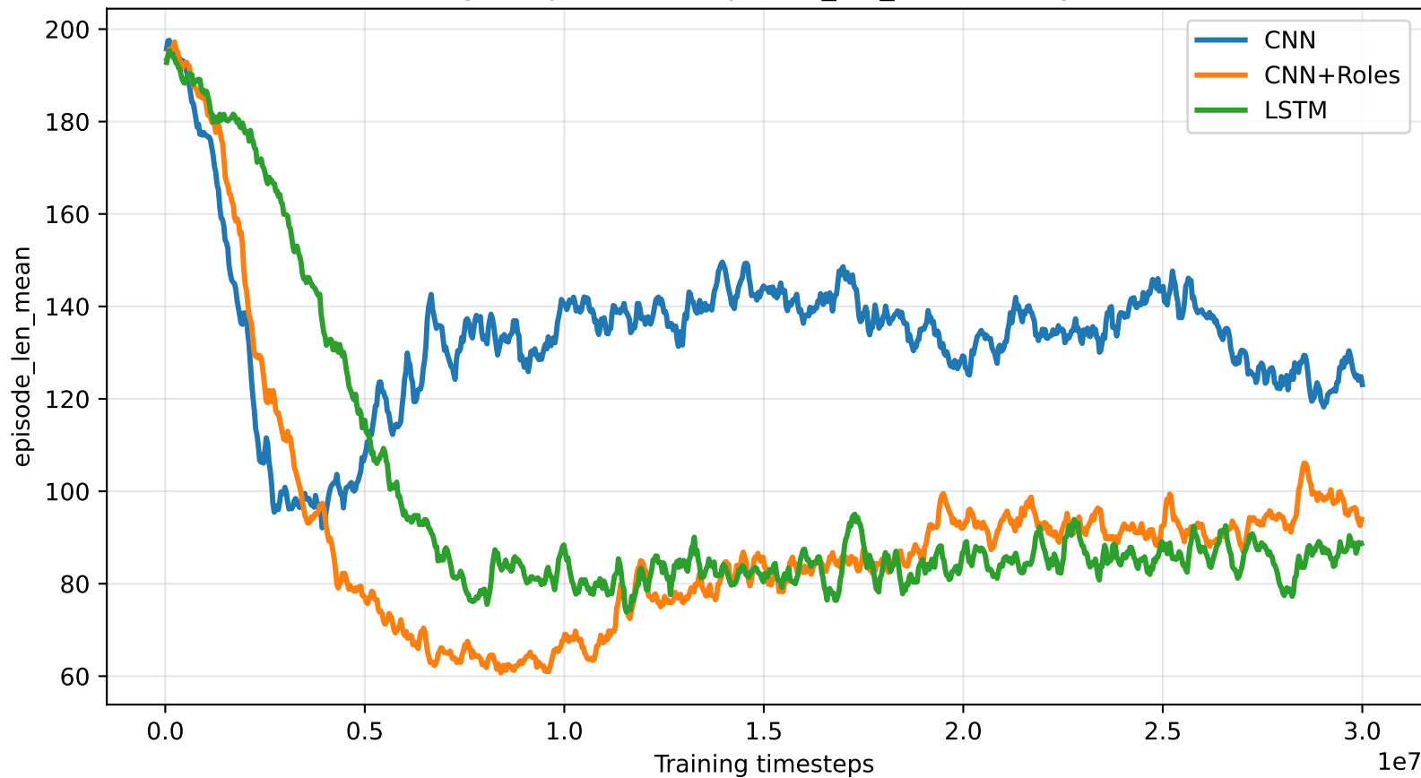
Training comparison:S6 episode_len_mean rolling mean
