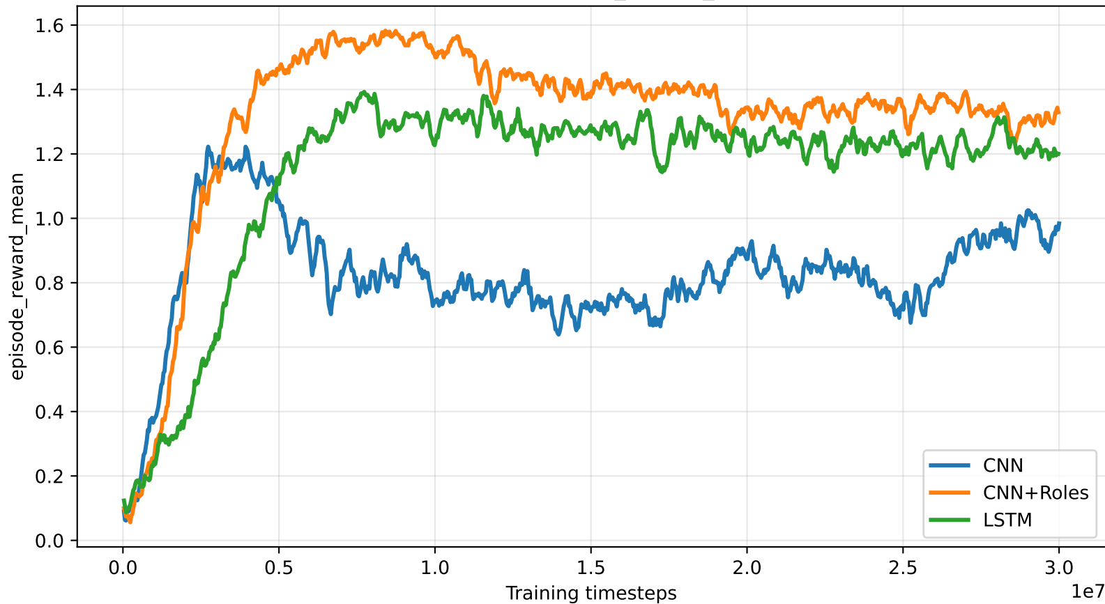
Training comparison:S6 episode_reward_mean rolling mean
