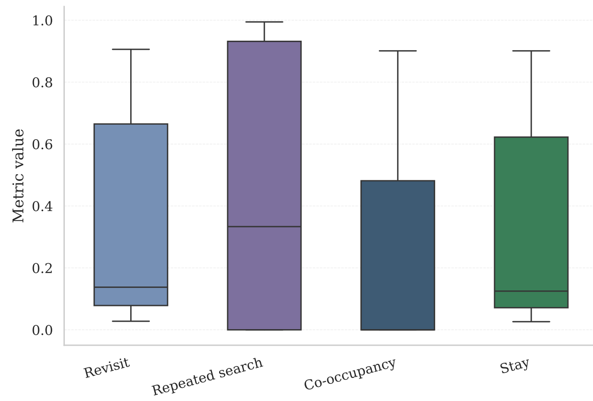
Coordination Metrics
