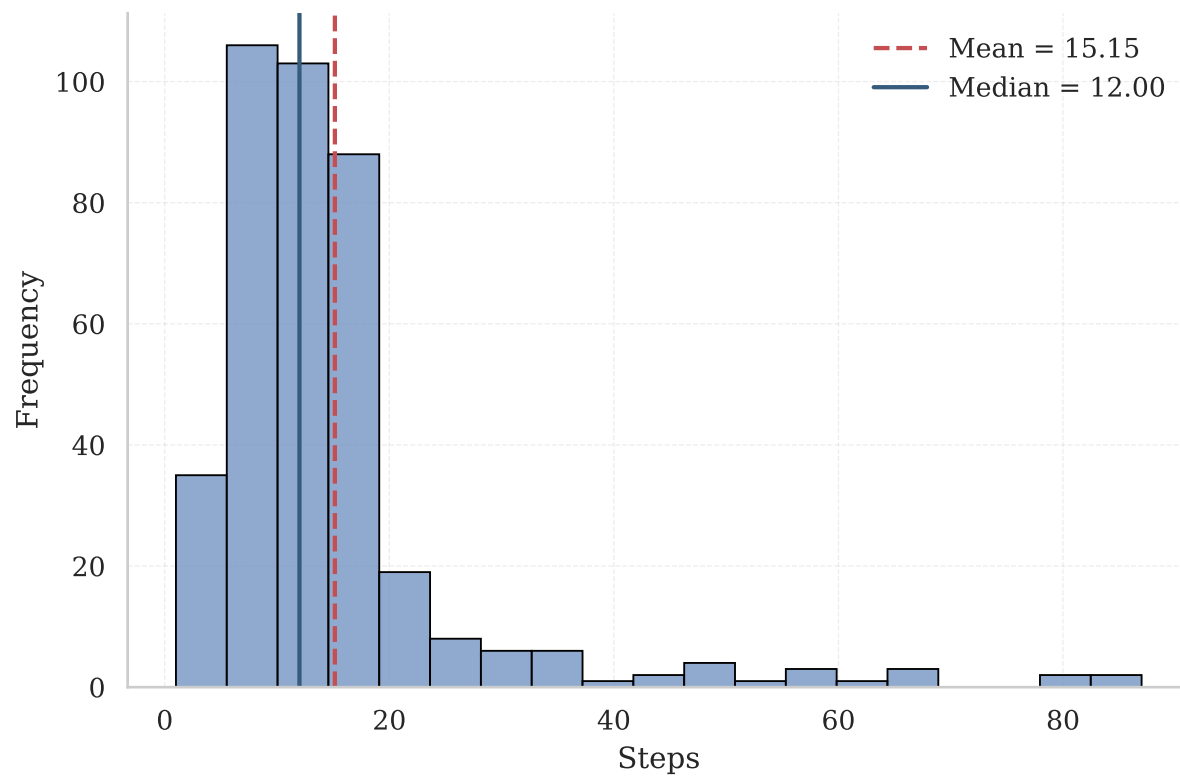
Coordination Metrics
