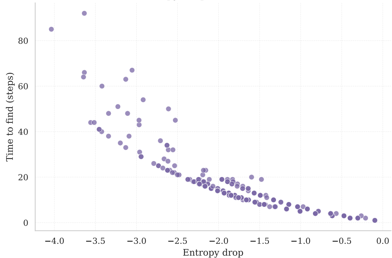
Entropy Drop vs Time to Find
