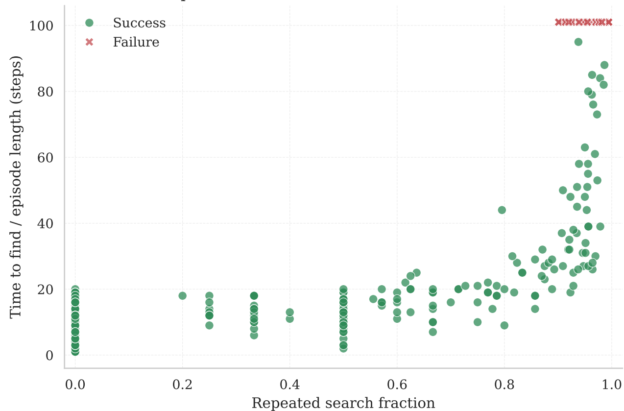
Repeated Search Fraction vs Search Outcome
