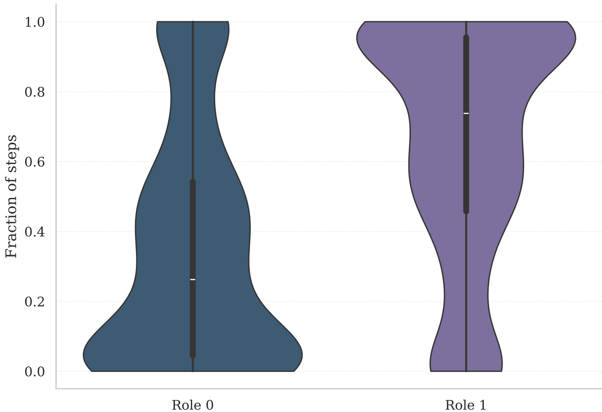
Role Usage Fraction per Episode
