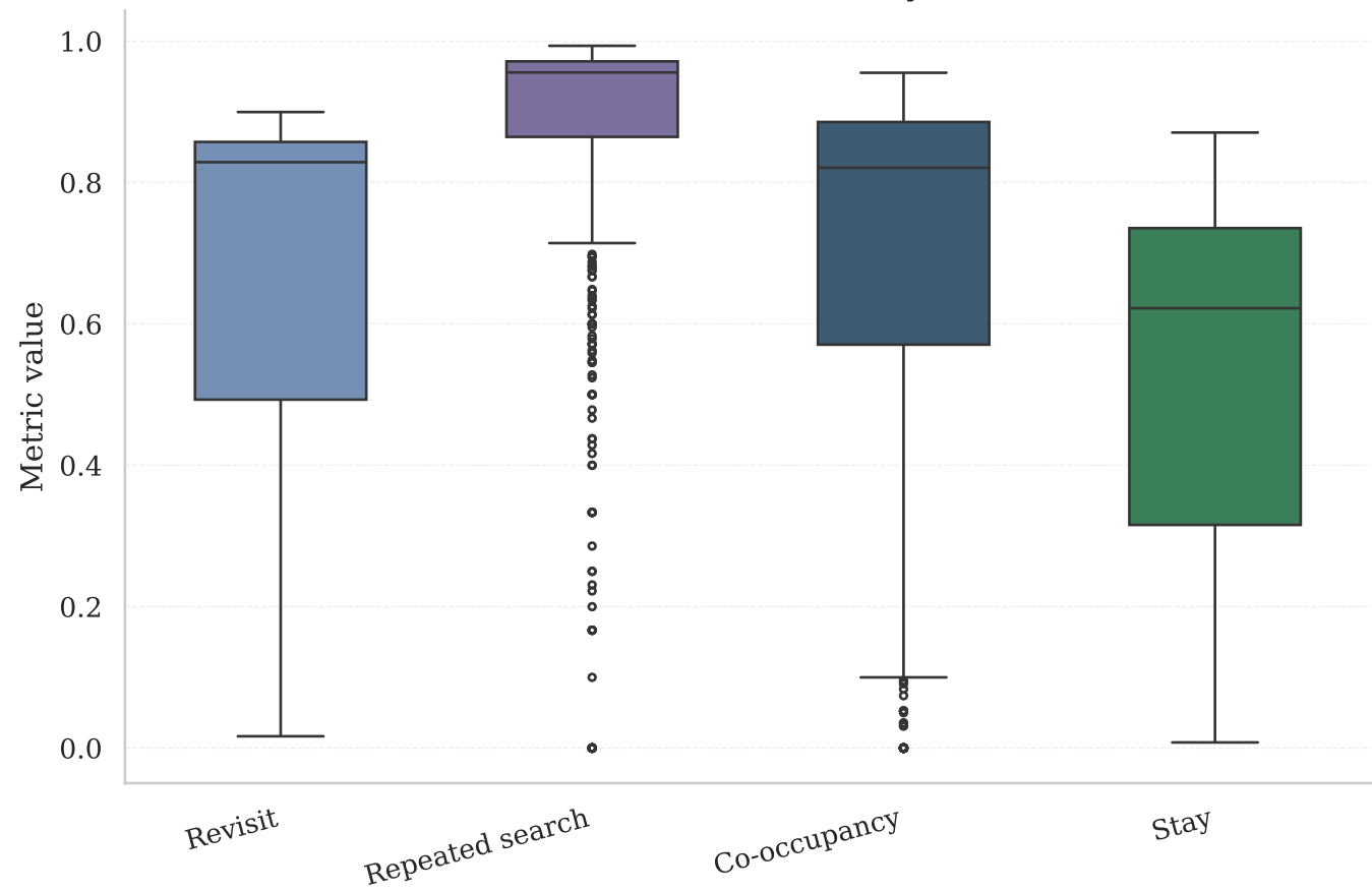
Coordination and Inefficiency Metrics
