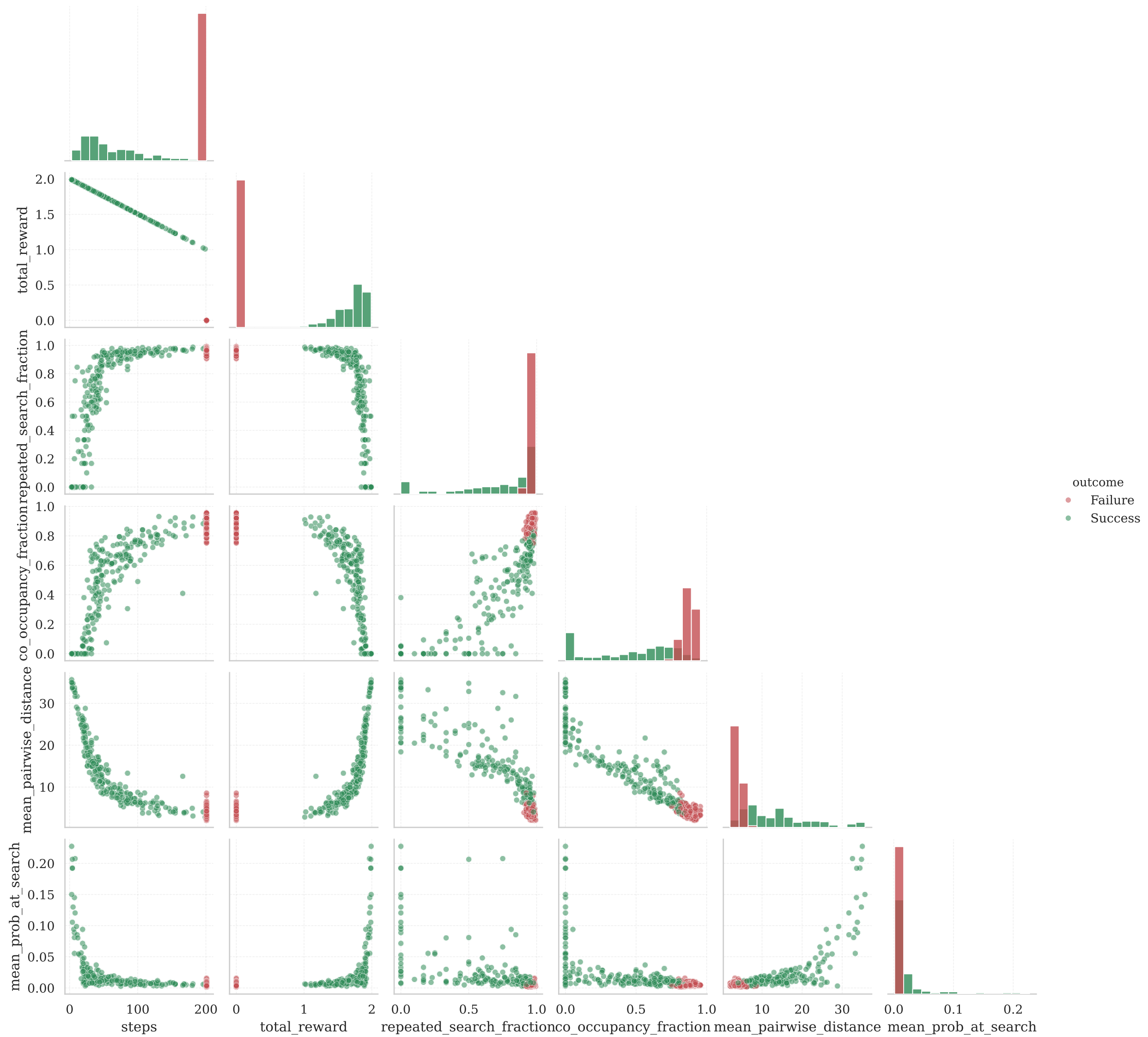
Pairwise Relationships of Selected Metrics
