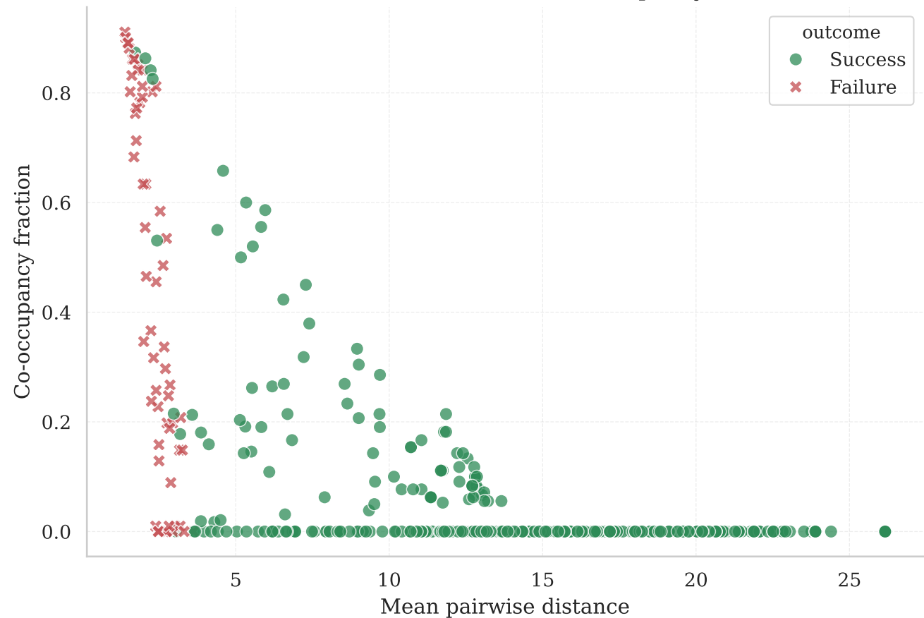
Pairwise Distance vs Co-occupancy
