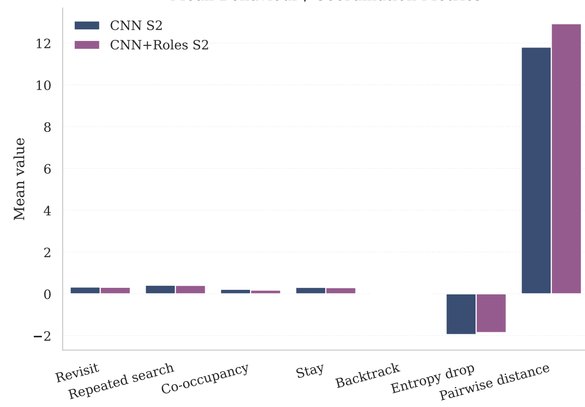
Mean Behaviour / Coordination Metrics
