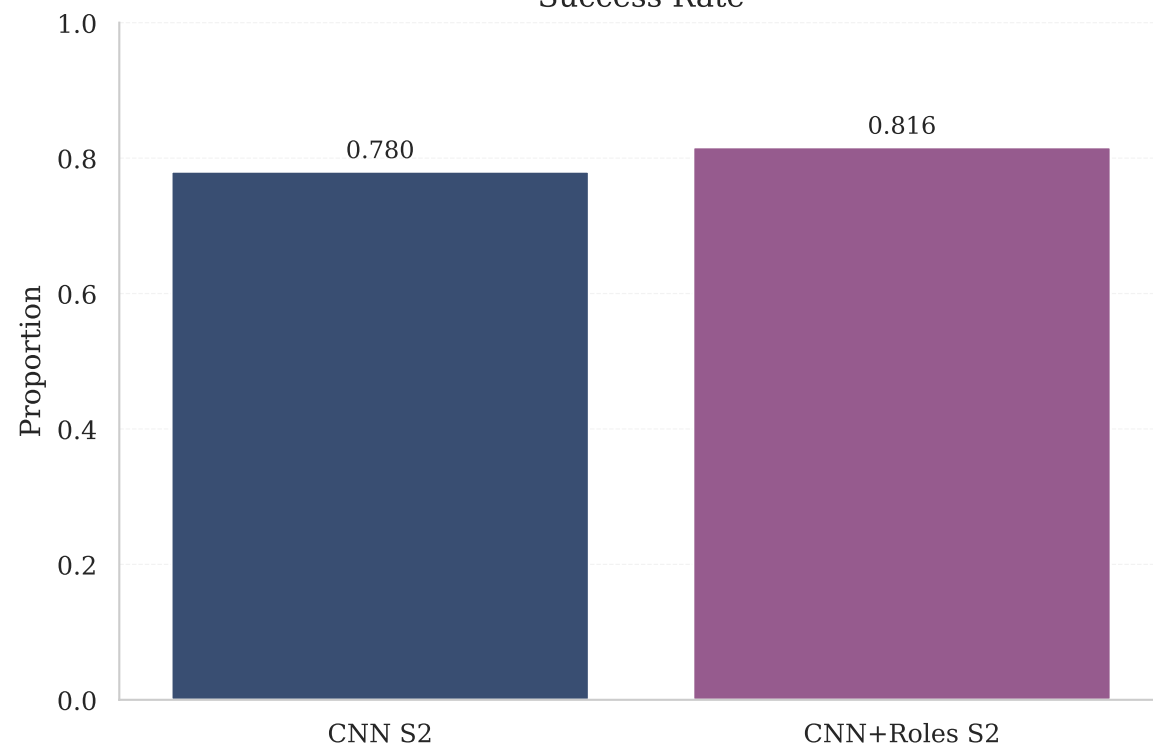
Success Rate
