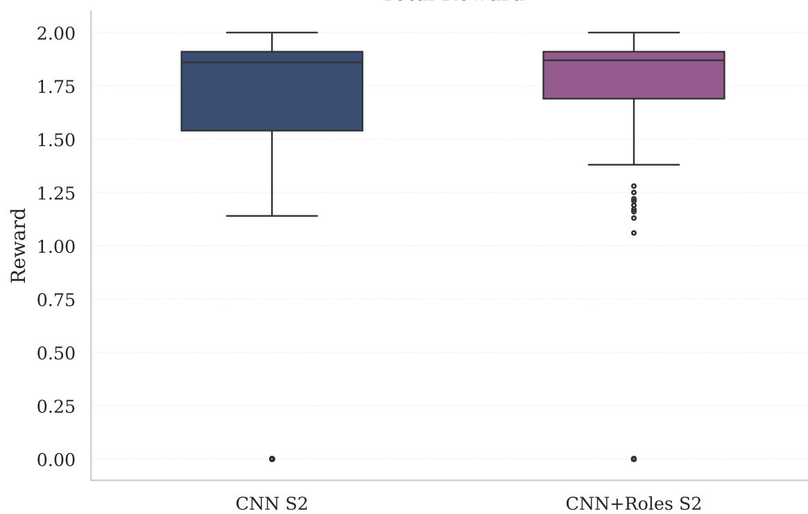
Total Reward
