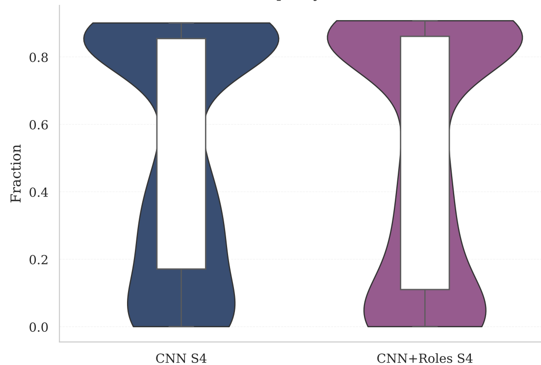
Mean Pairwise Distance
