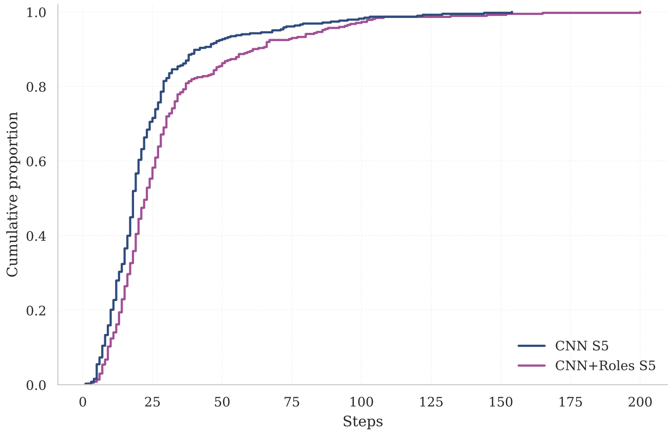
ECDF of Time to Find
