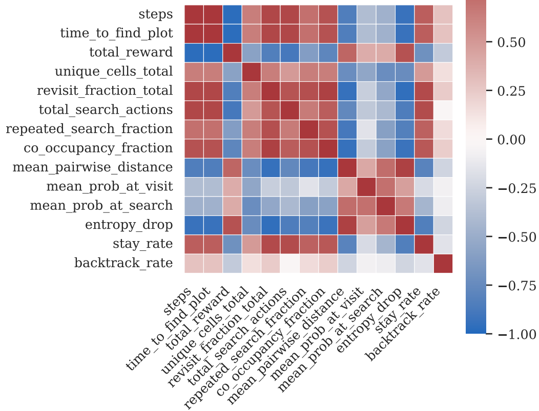
Correlation — CNN+Roles S6
