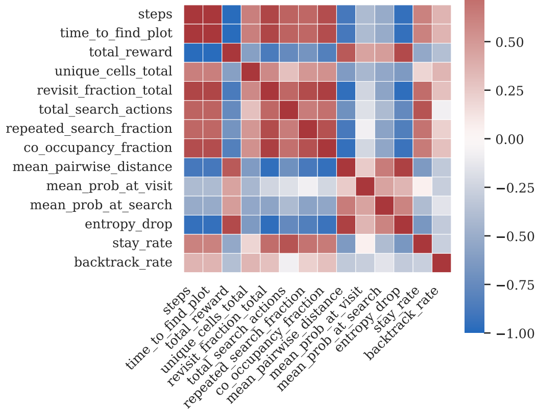
Correlation — CNN S6
