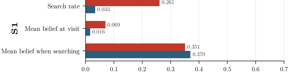
searcher role 1 (82%) · explorer role 0 (18%)
