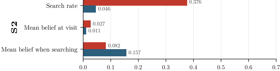
searcher role 0 (69%) · explorer role 1 (31%)
