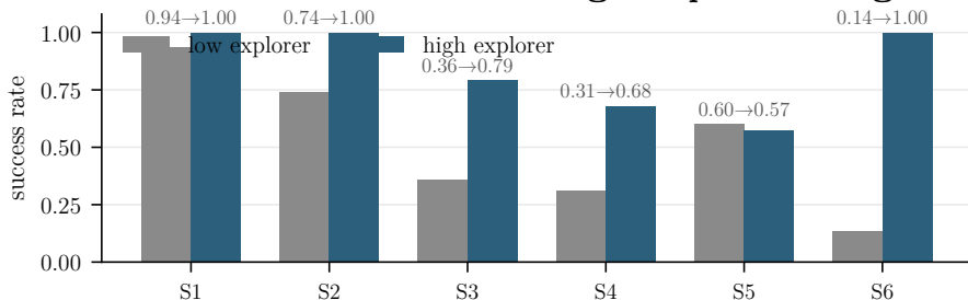
4. Success under low vs high explorer usage
