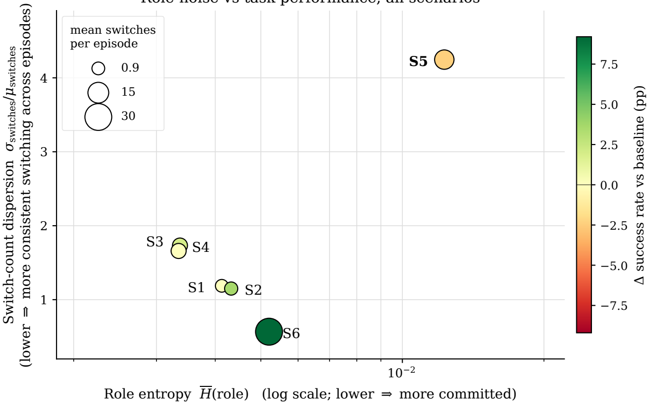
Role-noise vs task-performance, all scenarios
