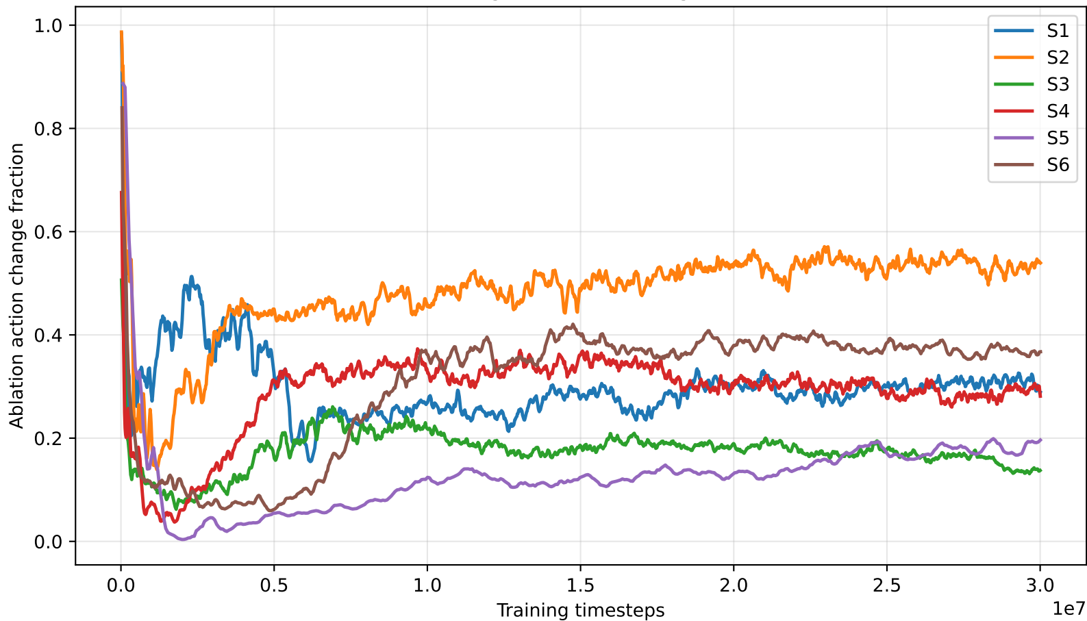
Ablation action change fraction (rolling mean, window=5)
