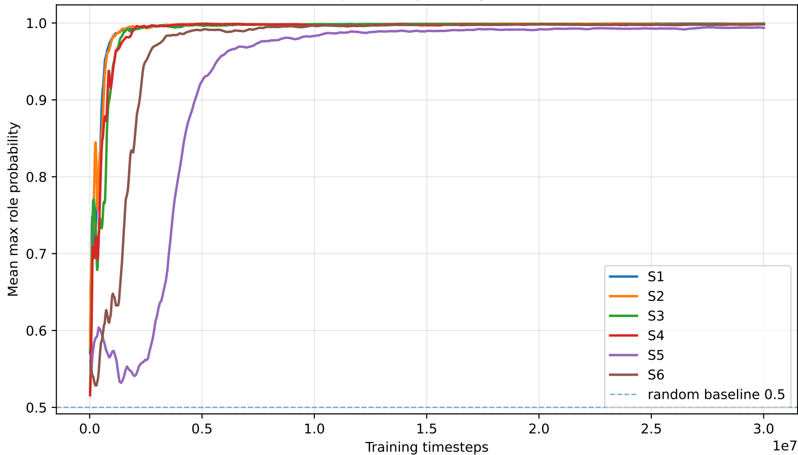
Mean max role probability (rolling mean, window=5)
