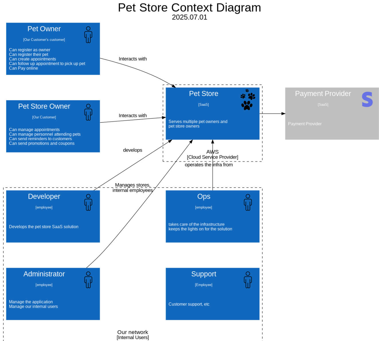
Figure 1: Context Diagram
