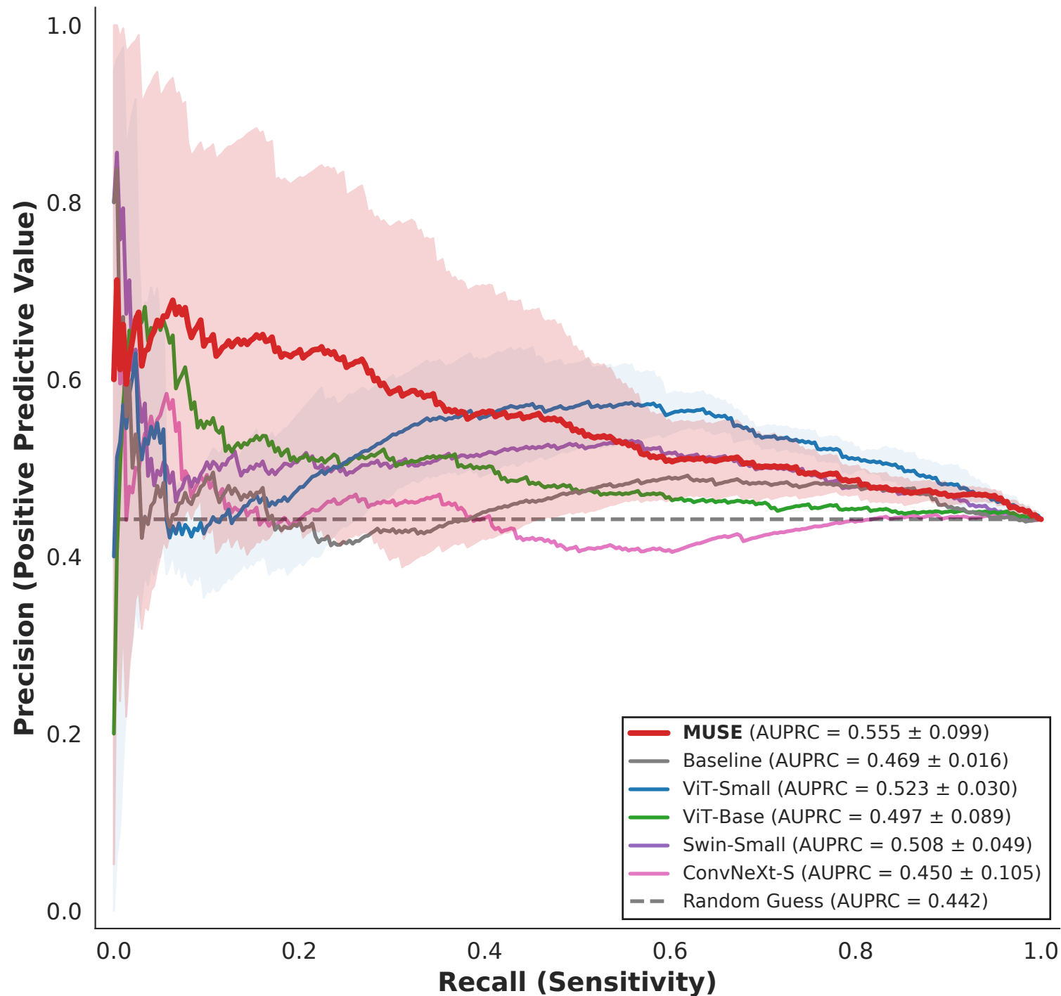
(A) External Multi-Center Evaluation PR Curves
