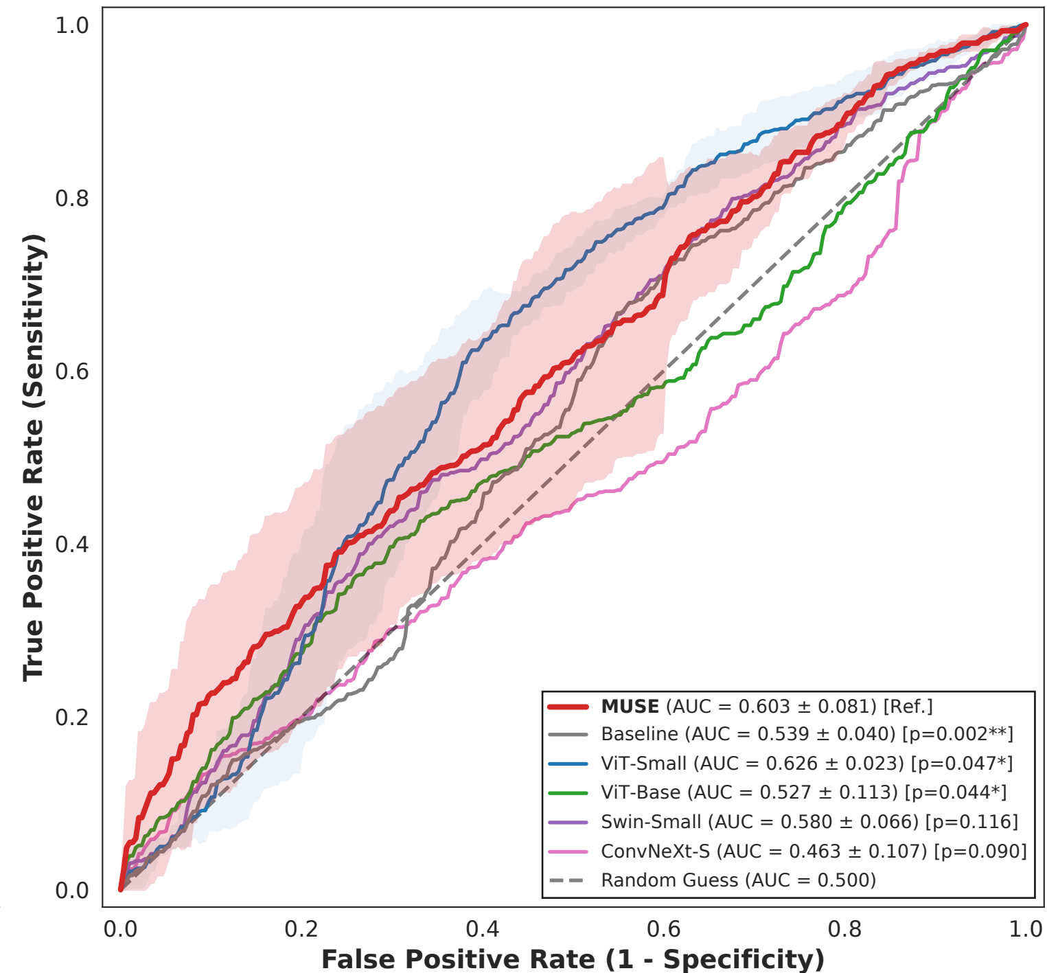
(B) External Multi-Center Evaluation ROC Curves
