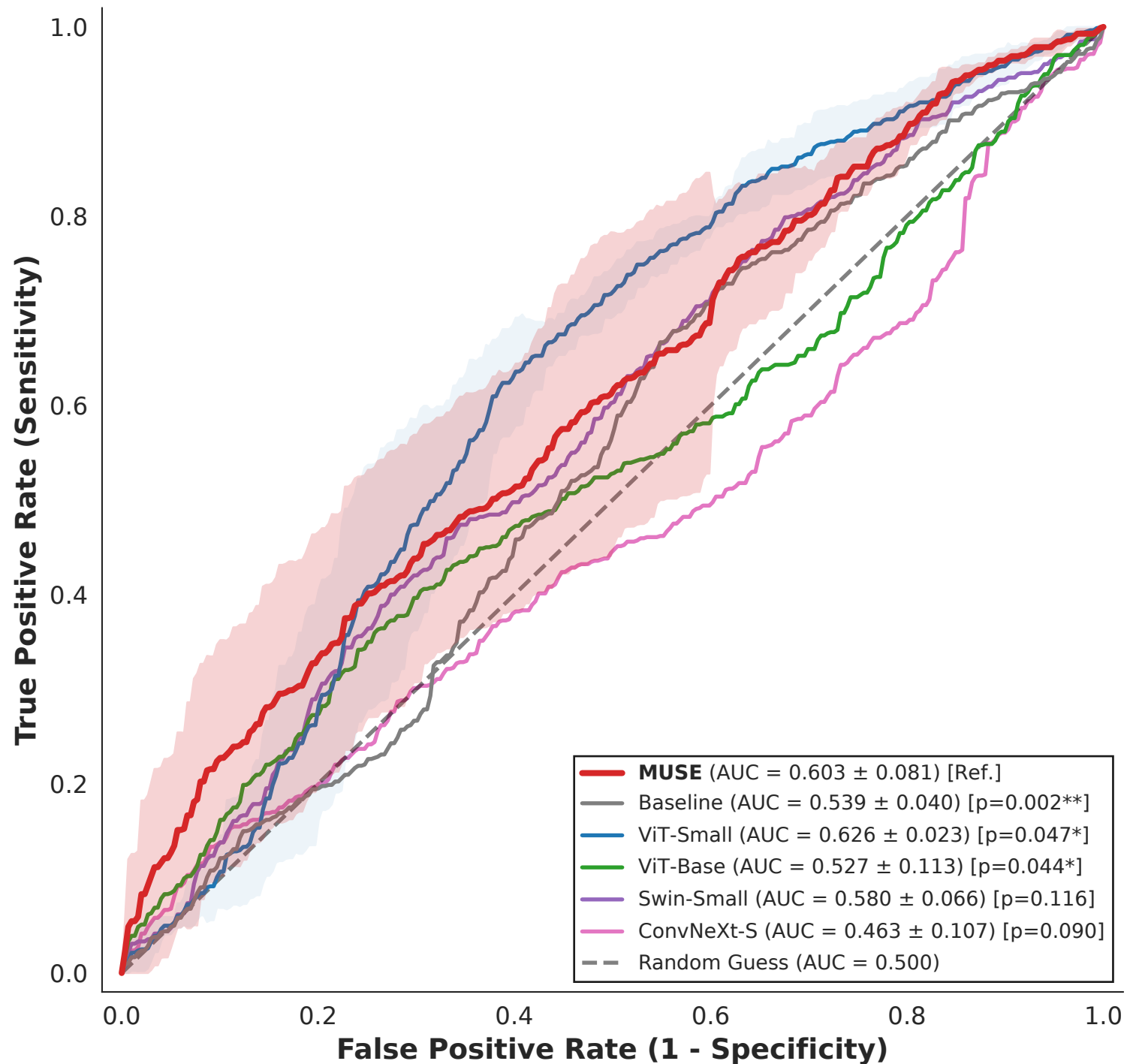
(A) External Multi-Center Evaluation ROC Curves
