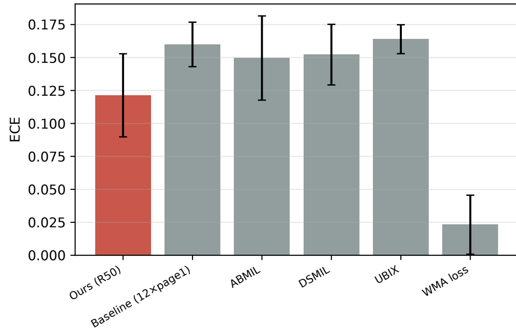
ECE (Ext pooled) ↓ better
