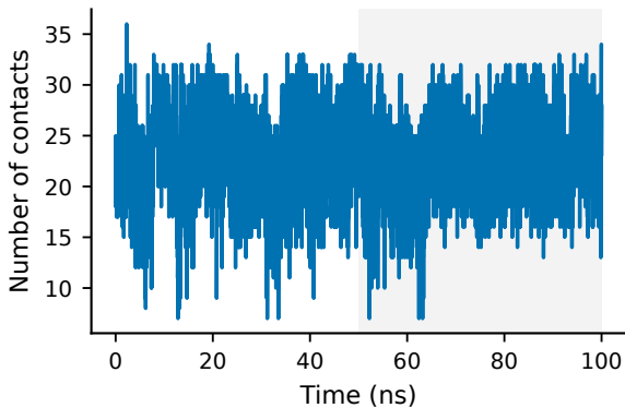
drugs2263 rep2
