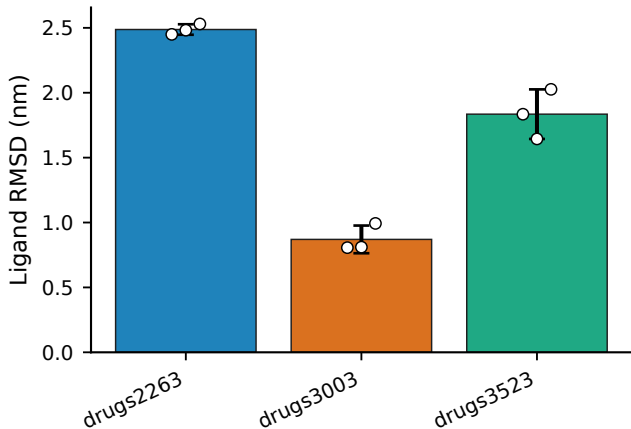
Ligand heavy-atom RMSD
