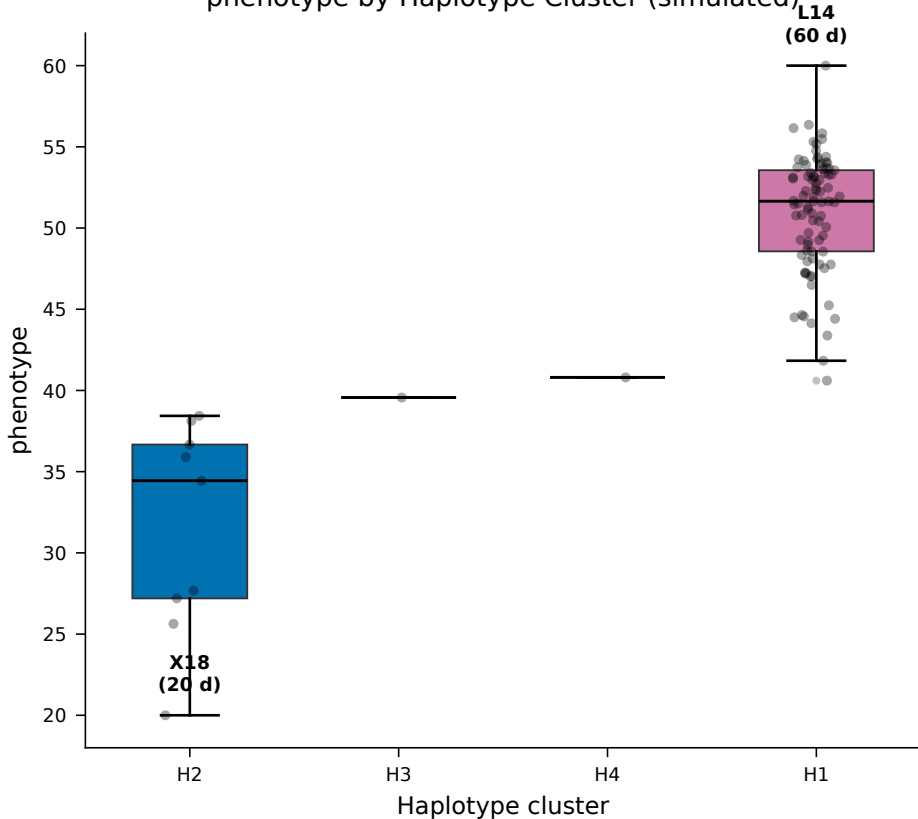
phenotype by Haplotype Cluster (simulated)
