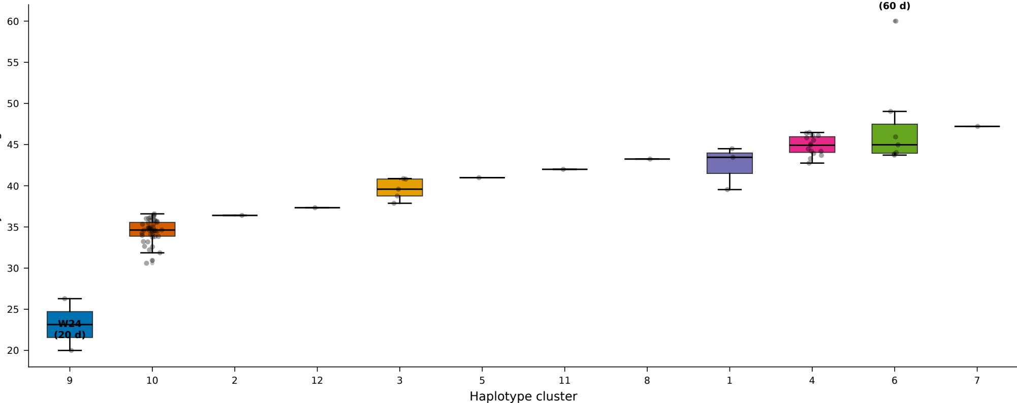
Days to flowering by Haplotype Cluster (simulated)
