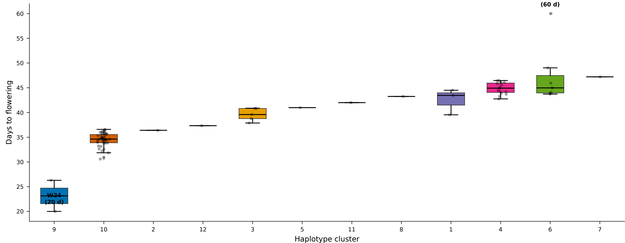
Days to flowering by Haplotype Cluster
