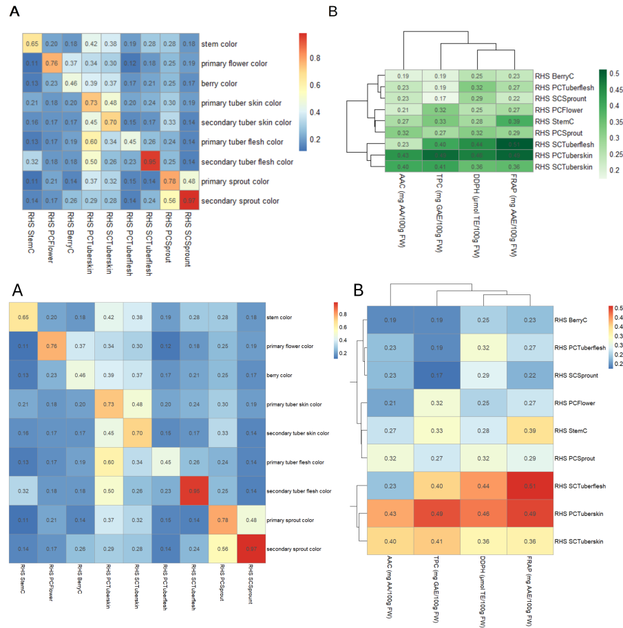
Figure 3 Correlation and determination coefficients of RHS potato color traits in CCC accessions. A. Heatmap showing the correlation matrix of potato color traits in CCC accessions, derived from descriptors by Gómez (2000) and measured with RHS (Voss, 2002) color chart. The color bar is located in the top right, with blue indicating low correlation values and red representing high correlation values. B. Heatmap showing the determination coefficient between nutritional (AAC) and nutraceutical (TPC, DPPH, and FRAP) assay reported by (Berdugo-Cely et al., 2023) components and potato RHS color traits. The color bar is located at the top right, with the intensity of green representing the determination coefficient.
