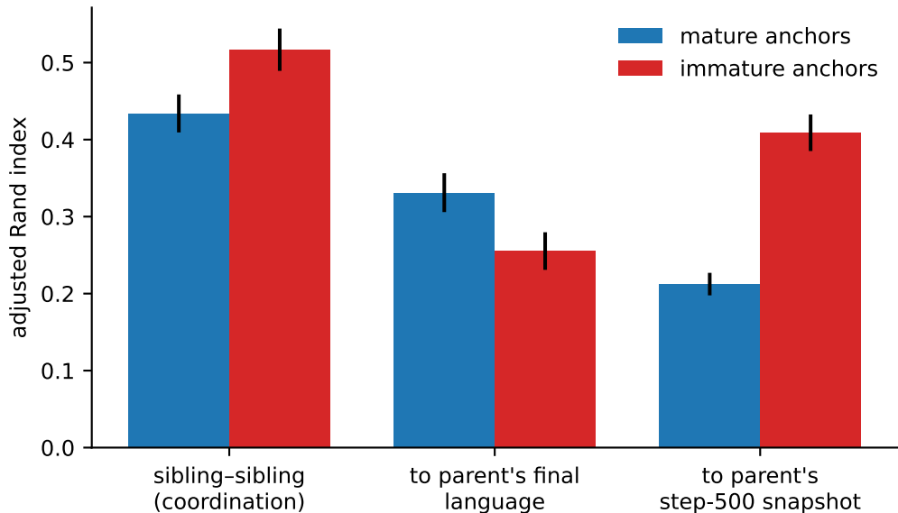
Coordination strength vs target (K17a/K17c); n=45: 30 discovery + 15 pre-registered
