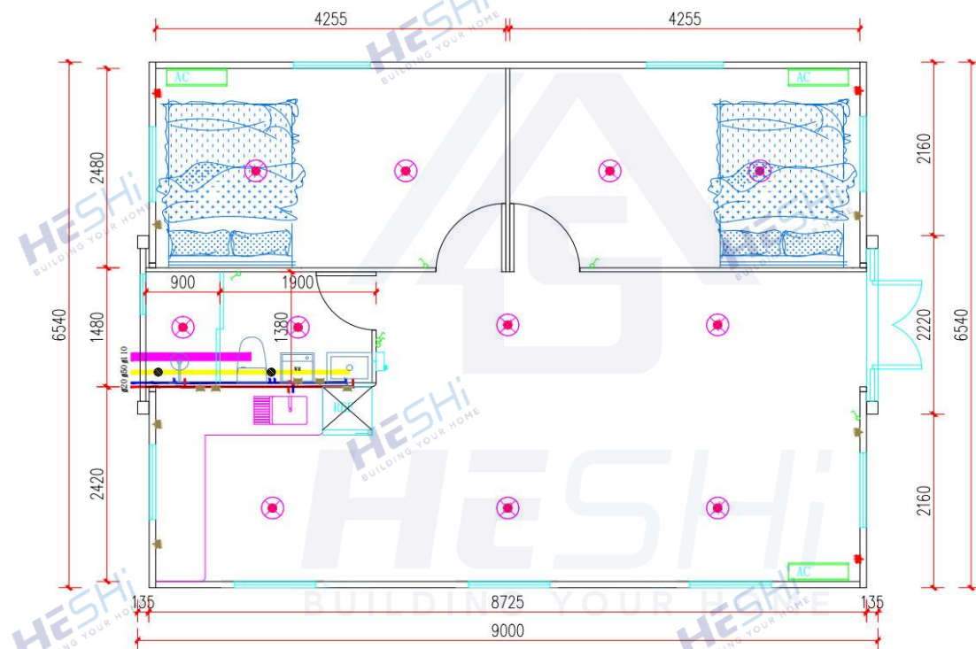
Ground floor plan /SIDE-30FT
