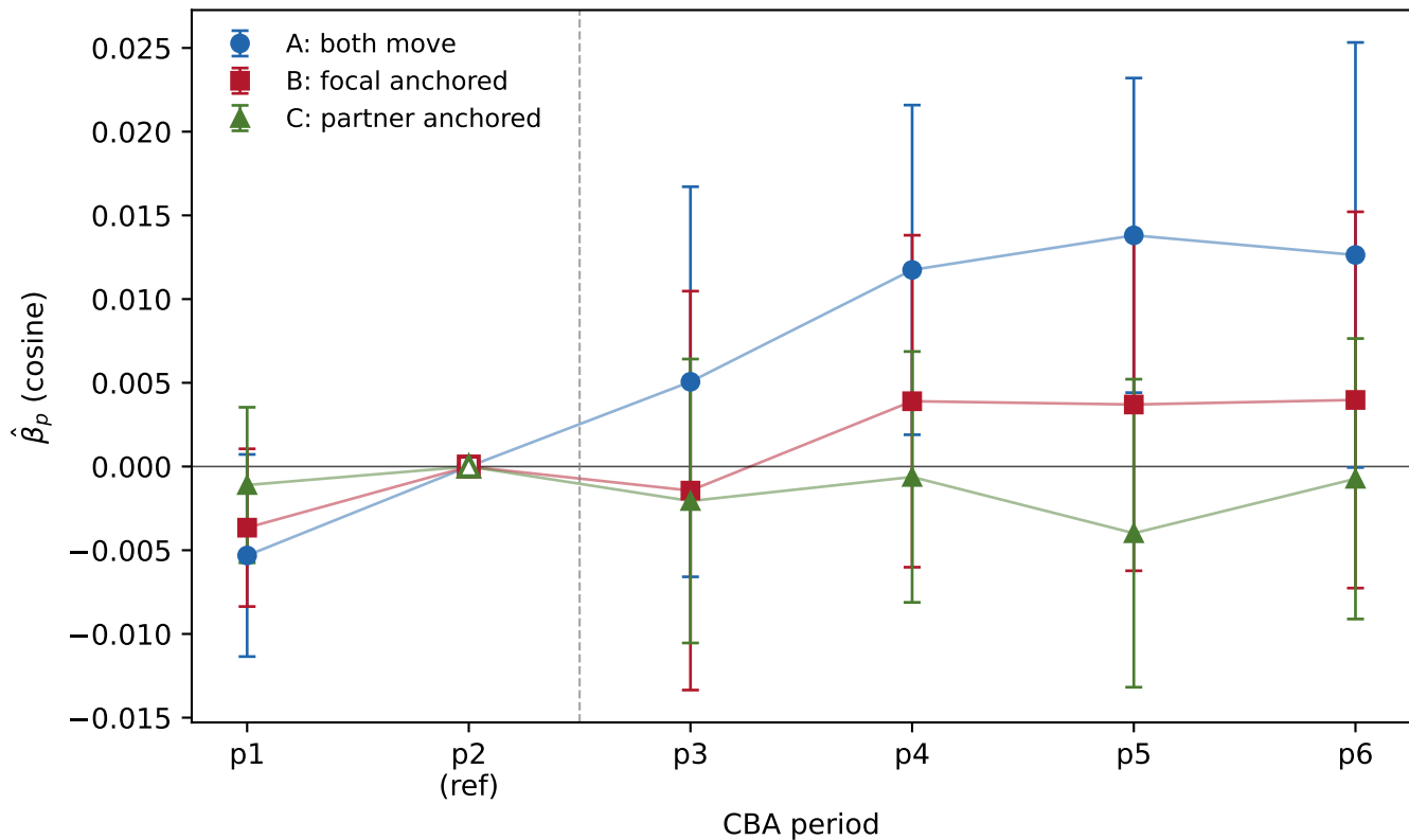
Cosine similarity
